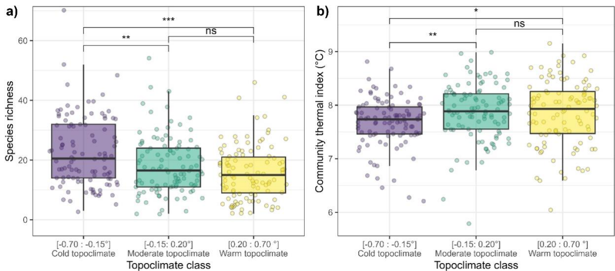
Figure 3 - Species richness a) and community thermal index b) of 306 floristic surveys evenly spread into three topoclimate classes of even number of plots (n=102 species by class). The p-value significance of a Wilcoxon test between two classes is displayed as follows: (ns): p > 0.05 (*): p < 0.05 (**): p < 0.01 (***): P < 0.001 .
