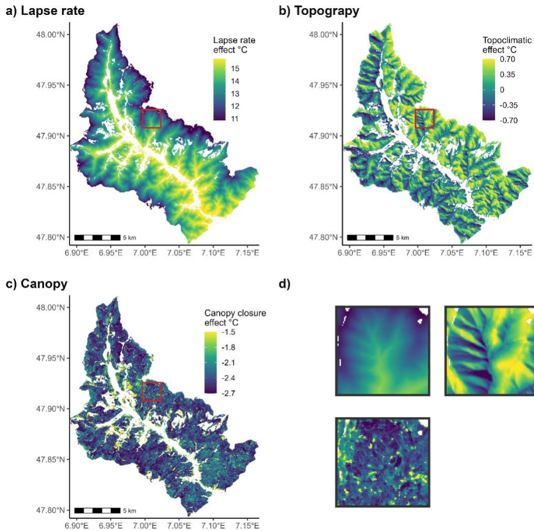
Figure 2 - a) Elevation induced change in mean growing season understory temperature of the growing season (lapse rate of -0.68^{\circ}\text{C}\cdot 100\text{ m}^{-1} ), assuming a canopy closure of 90% and no effect from topography. b) mean understory temperature effect induced by topography (heat load and topographic position, i.e. topography) assuming an average canopy cover (90%), compared to a moderate situation (flat terrain midslope). c) mean understory temperature cooling induced by canopy closure assuming no effect from topography. For visualization purposes only we restrained the minimal cooling to -1.5^{\circ}\text{C} , however some pixels displayed lower values up to 0^{\circ}\text{C} due to low canopy closure. d) 2 km per 2 km zoomed inset of the red square of the other panels, their color gradient corresponds to the color scale presented in the other panels a-c, respectively. Blank pixels represent land covers other than forests or forests outside of the study region. Linear model R^2 : 92.2%.
