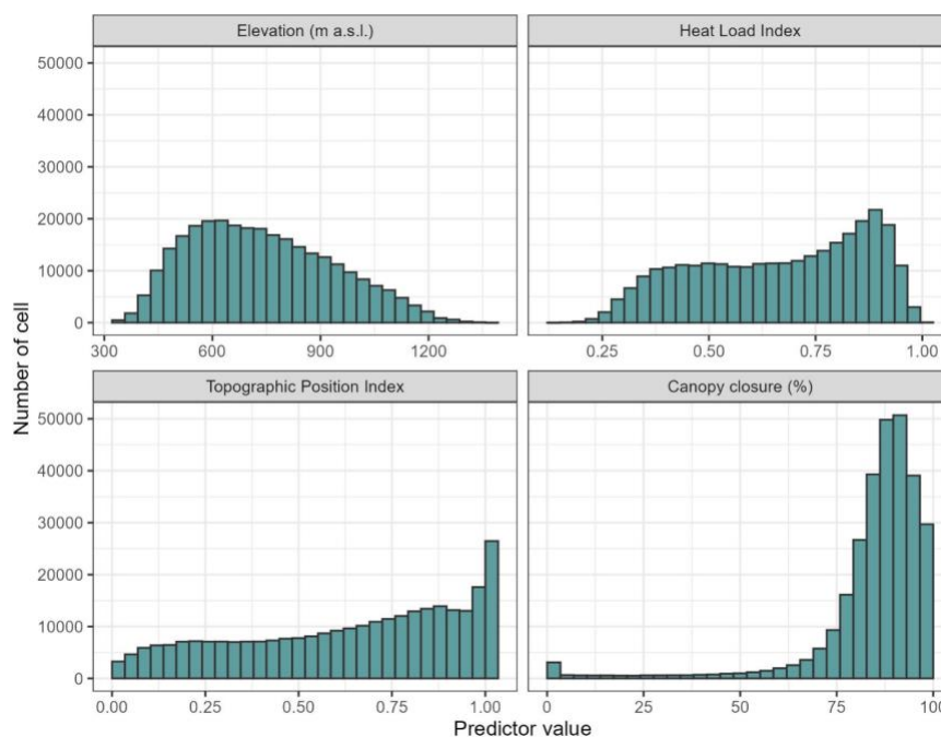
Figure S1: Distribution of the value of the four tested predictor of understory temperature through all the cells of the study region (forested cells of the Thur valley).
