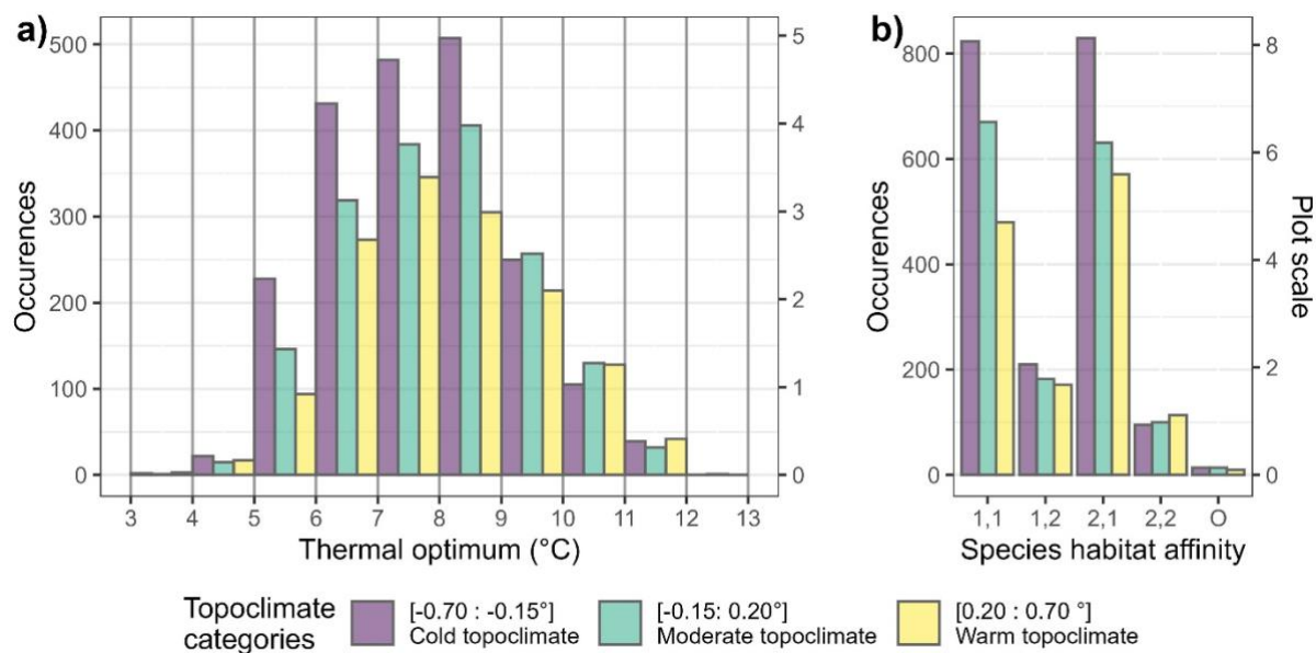
Figure 4 - Occurrences of species in the three topoclimatic classes as a function of a) their thermal optimum (°C) and b) their habitat affinity defined by the EuForPlant list as follows: 1,1: closed forest mainly 1,2: forest edges and opening 2,1: forest and open vegetation 2,2: mainly in open vegetation (Heinken et al. , 2022) The plot-scale occurrence of species is also shown (e.g., 400 occurrences corresponds to approximately 4 species per plots).
