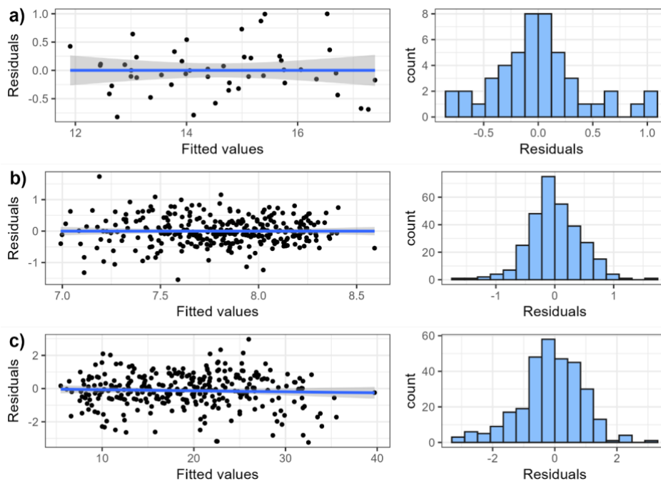
Figure S6: Relationship between residuals and fitted values, and histogram of residuals of the linear mean temperature model (a), the CTI linear model (b) and the species richness negative model (c).
