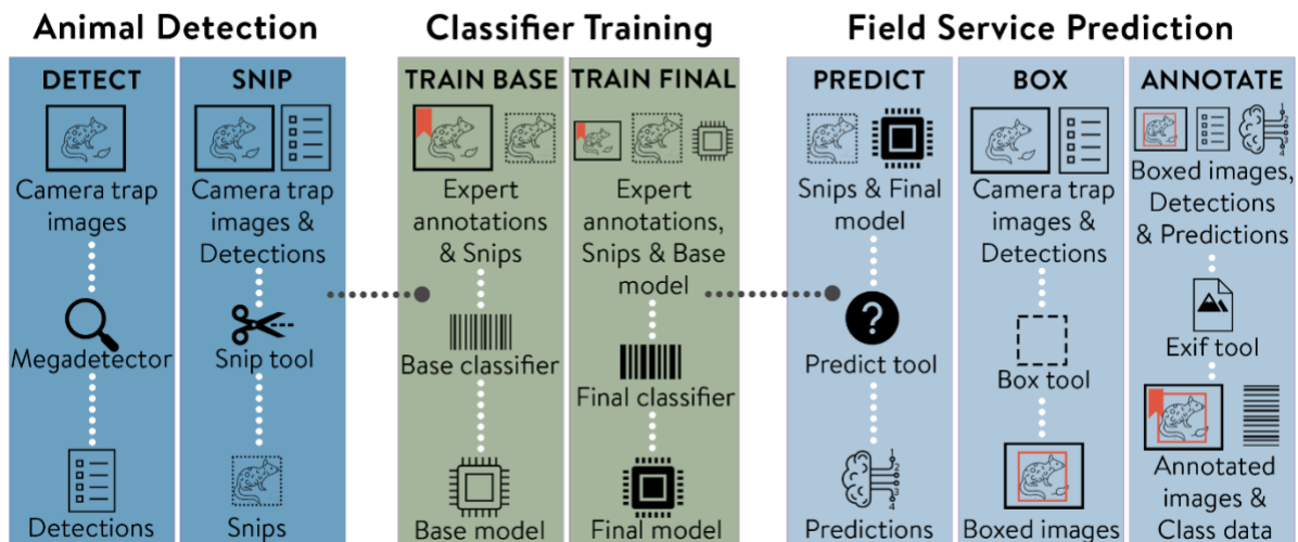
Figure 1 - The MEWC workflow. Each step in the camera-trap-image processing pipeline has an associated Docker container. The Expert Annotations (species labels for the training images) provide the basis for building a supervised classification model (see Appendix details on this step). Detection data are combined with prediction data (inferred from the classifier) to produce the red-boxed images and final classification data. The classification data includes basic information written to metadata fields of the images, and a detailed CSV file (one image per row) that can be used for direct analyses or import into a dedicated camera-trap database like Camelot for rapid expert validation.
